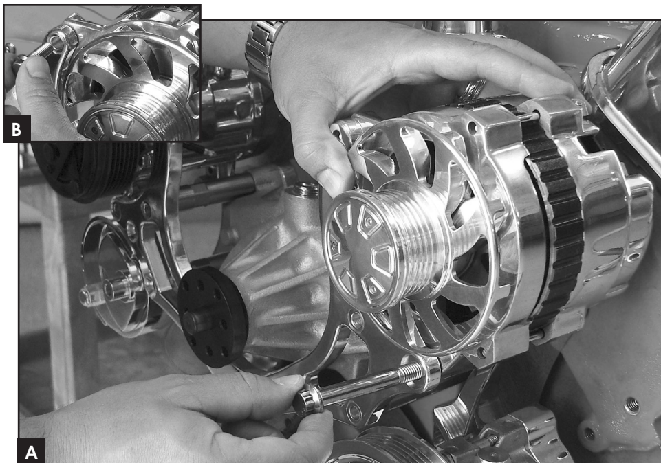
Figure 10: Attaching Alternator
