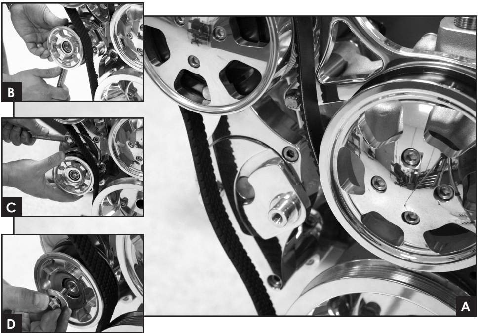
Figure 14: Install Serpentine Belt & Tensioner Pulley
