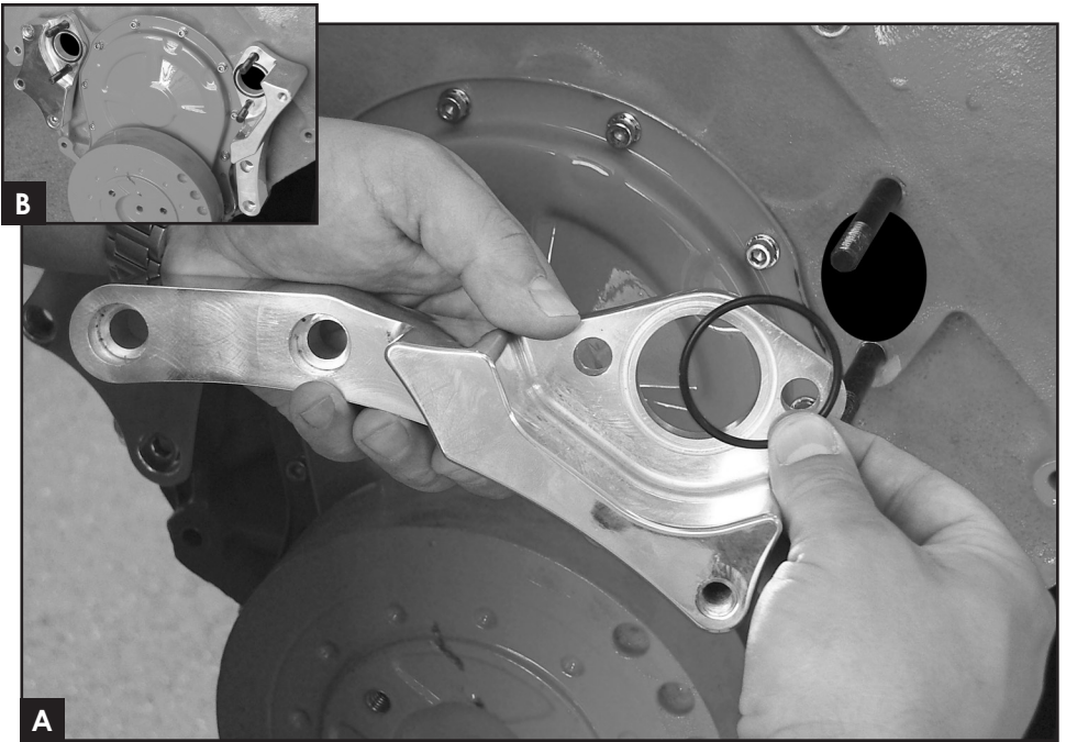
Figure 3: Install Alternator Bracket
