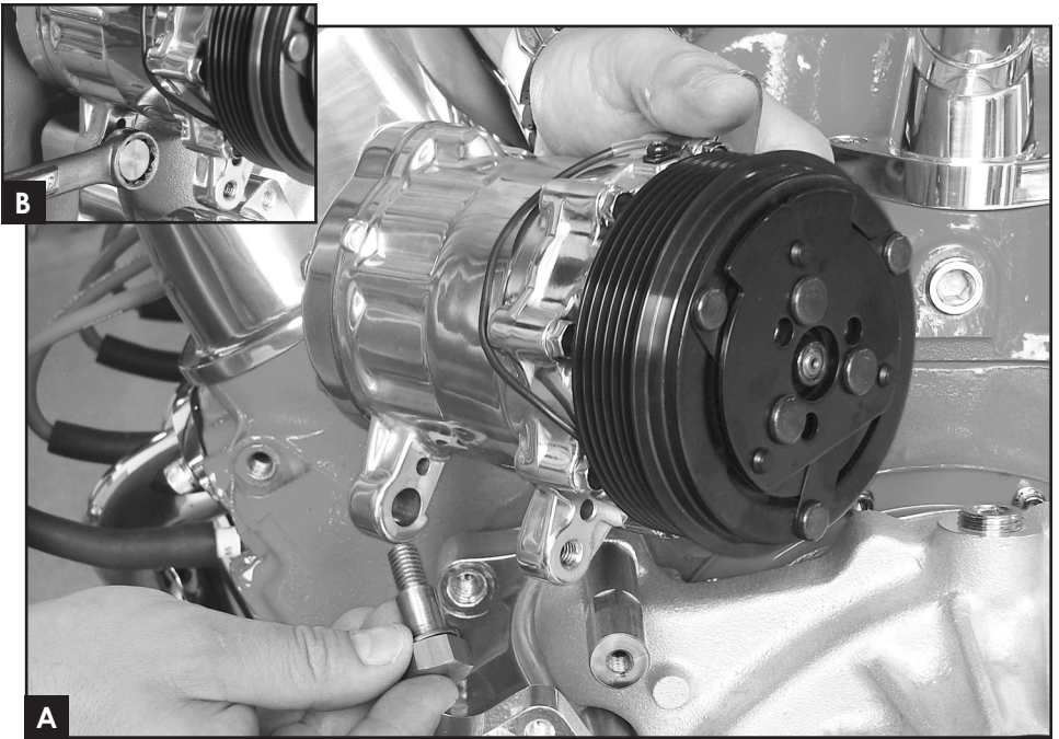
Figure 8: Install SD-7 Compressor
