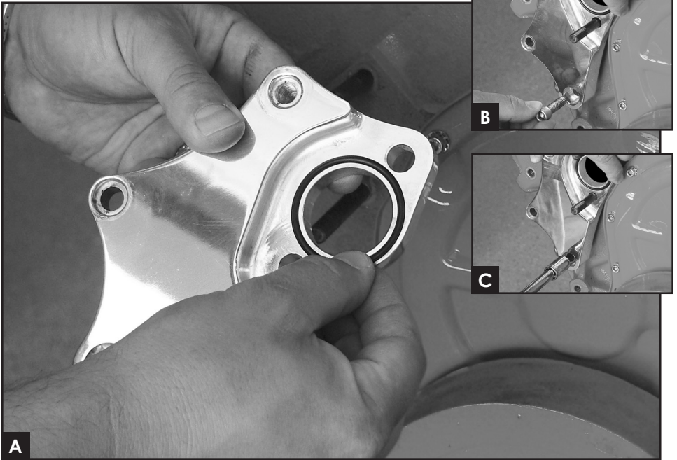
Figure 2: Install O-Rings & Compressor Bracket
